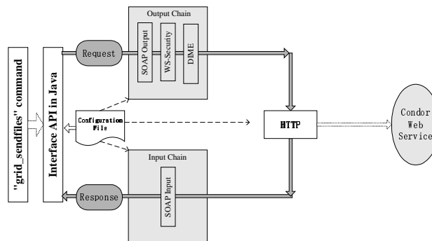
Figure 1: Implementation of Data Upload with the Message Filter Chains
